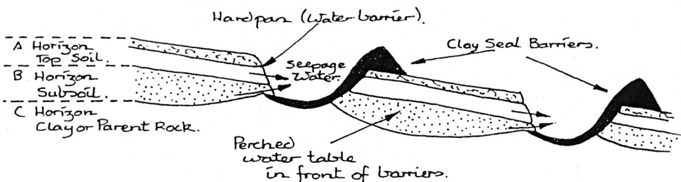
Figure 9.18 Interceptor banks have to be cut into the clay layer to prevent water from seeping downslope. The water can be used upslope -it moves through the soil by capillary action - or taken to a dam or safe disposal site.
