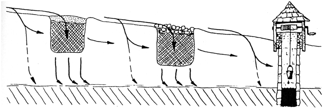
Figure 9.25 A pit filled with compost and covered in stone or sand can trap and store water. Natural seepage and drainage of water will slowly fill pits and wells.
