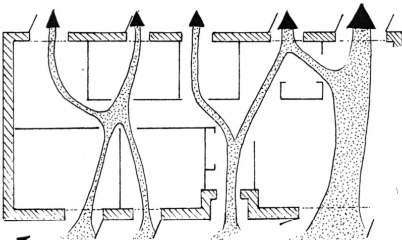
Figure 8.5 A solar chimney is one way to cool the interior of a house. Air is drawn from below the house, often across water, and ducted through the house and then vented.
