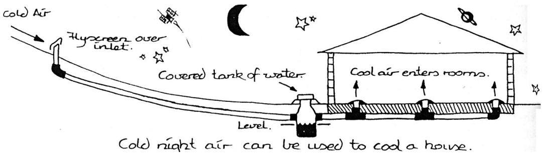
Figure 8.4 Cold night air is cooled as it passes over water before it is ducted into the house.
