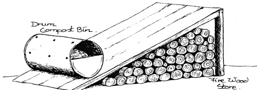
Figure 10.1 Use a 200 L (44 gal) drum as a compost turning device.
