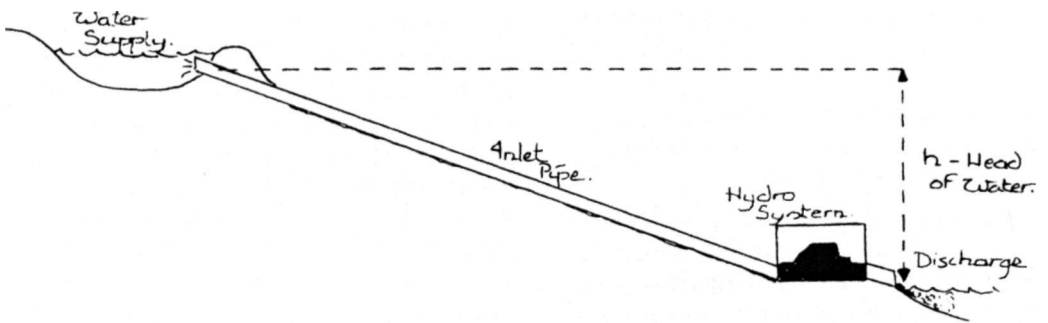
Figure 14.7 The head of water is the vertical height of the water column.
