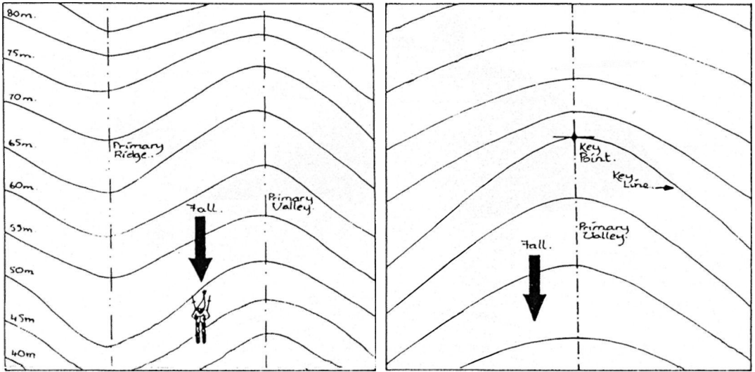
Figure 9.7 Contours, ridges and valleys in the landscape. The keypoint is found by looking at the changes in slope.
