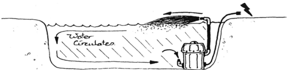
Figure 2.12 The submersible pump inlet should point upwards so that it does not draw in detritus material from the bottom.
