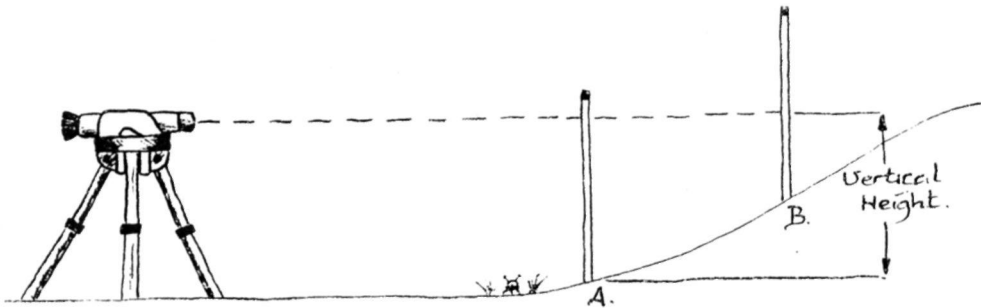
Figure 5.11 The difference between A and B gives the amount of rise in the slope.
