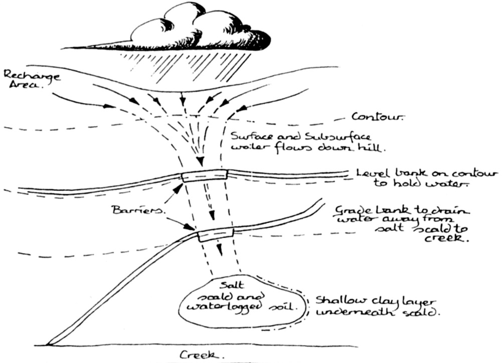
Figure 9.20 Clay-lined drains are barriers to water movement downslope. These drains can divert water from salt scalds and help to dry paddocks which waterlog easily.
