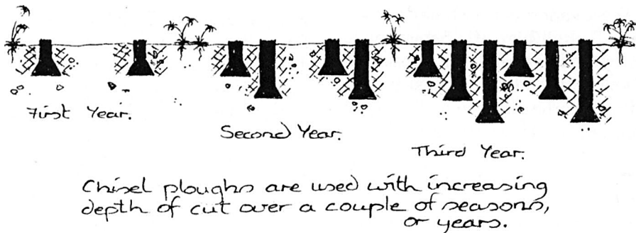
Figure 6.6 Chisel ploughs are used, with increasing depth of cut over a couple of seasons, on both small and large farms. This improves aeration and drainage, breaks up compacted soil and permits plant roots to penetrate deeper into the soil.
