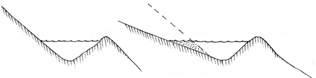
Figure 9.8 The higher the slope, the lower the storage ratio. The flatter the slope, the more water that can be stored efficiently.
