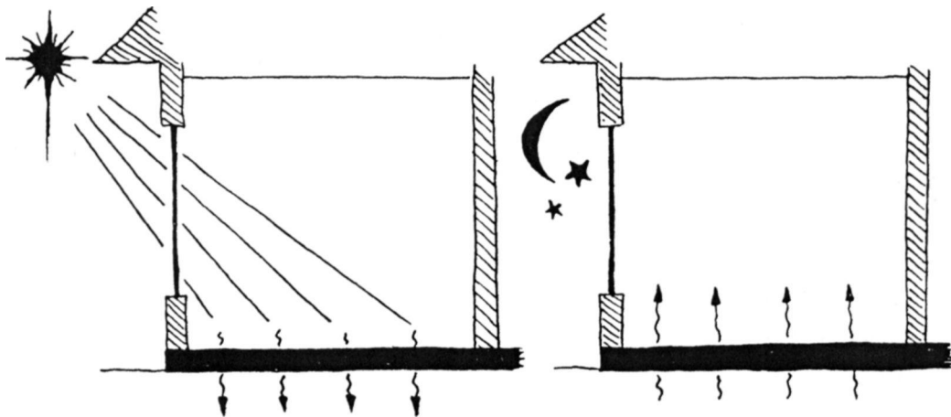
Figure 3.12 Floor radiating heat at night. Dark floors can absorb heat.
