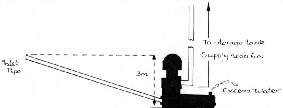
Figure 14.15 Hydraulic rams work day and night to pump water uphill to a storage tank.
