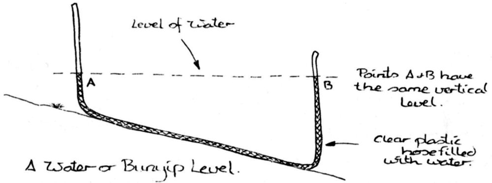
Figure 5.9 A simple Bunyip level made from plastic tubing.
