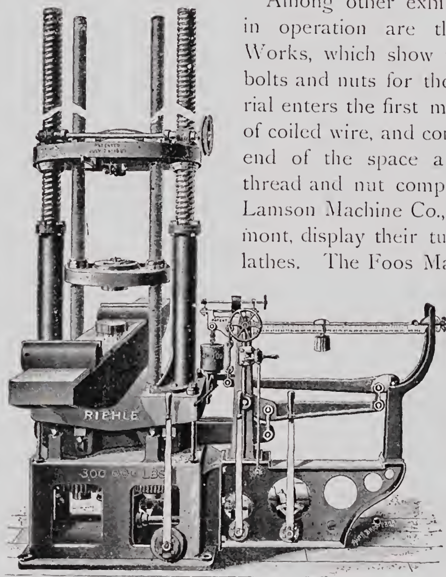
TESTING MACHINE. Exhibited by Riehle Bros.
