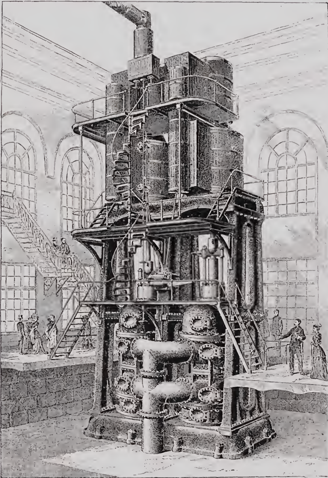
VERTICAL, PUMPING ENGINE—CAPACITY 40,000,000 GALLONS DAILY. Exhibited by Henry R. Worthington, New York.
