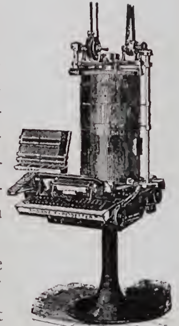
THORNE TYPE-SETTING MACHINE.
