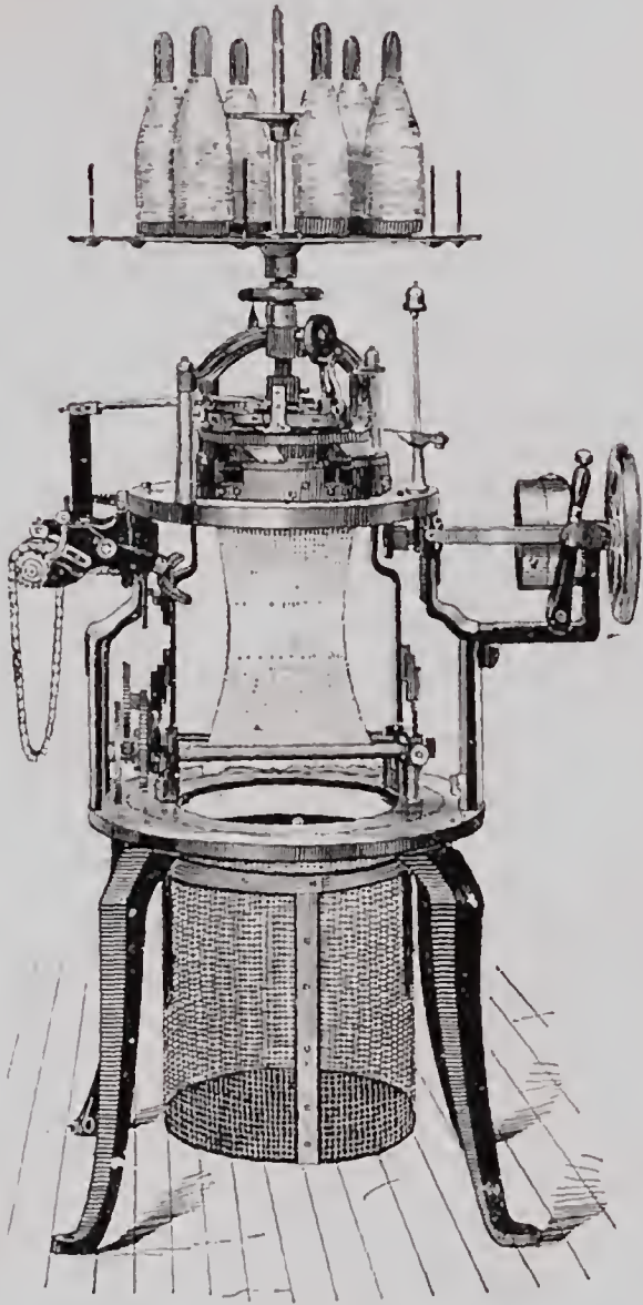
BALLOO RIBBED KNITTER. Exhibit of Lewis Jones.
