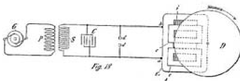
FIG. 18.—OPERATING A MOTOR BY DISRUPTIVE DISCHARGES.
