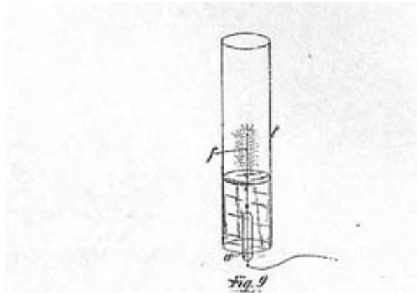
FIG. 9.—SHOWING THE EFFECT OF THE AIR.
