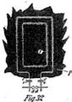
FIG. 32.—ELECTROSTATIC ACTION BETWEEN PRIMARY AND SECONDARY, WITH EXTREMELY HIGH FREQUENCIES.
