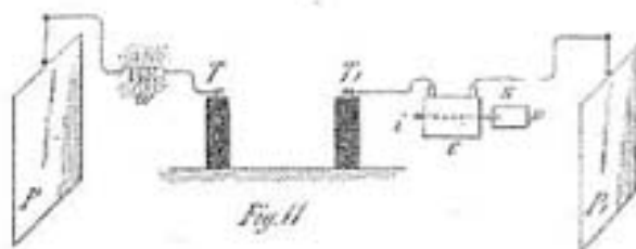
FIG. II.—SHOWING EFFECTS OF CURRENTS FLOWING THROUGH OPEN CIRCUITS.
