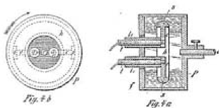
FIGS. 4a, 4b.—FORM OF DISCHARGER WITH LIQUID INTERRUPTER.
