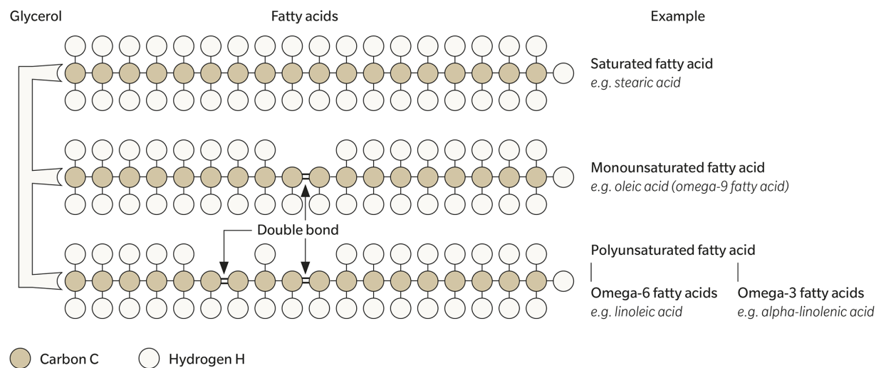
Fig. 11: Chemical structure of a triglyceride 131
