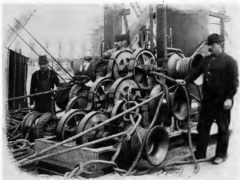
A Hoisting-Engine.
