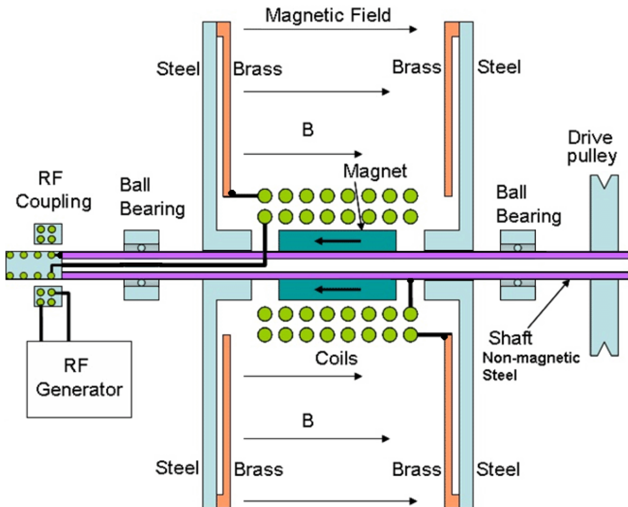
Fig.1 The cross-section of mechanical construction of the dual cyclotron-like device
