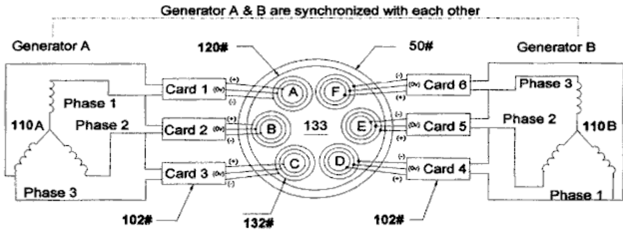
Configuration of Hydroxyl gas producing apparatus Fig-3
