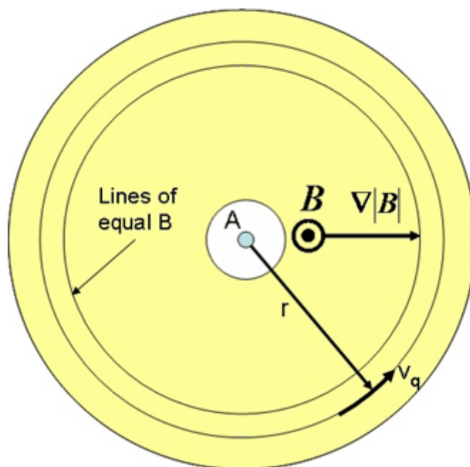
Fig.2. Gyration of the emitted charged particle in the gradient of the magnetic field in a brass disc under the condition of cyclotron resonance. The disc rotates in the opposite direction to the particles.
