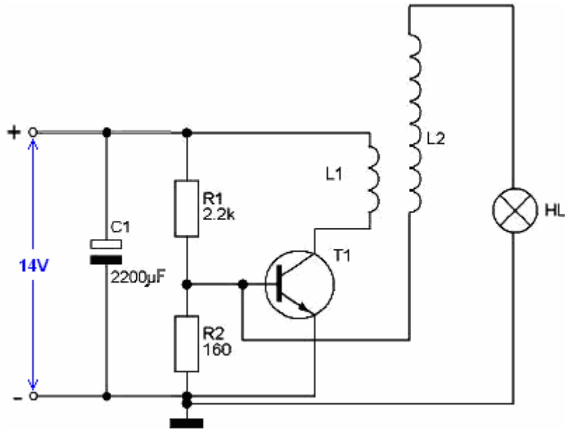
Fig. 3. Circuit of the experiment to determine the active power output of the L2 coil
