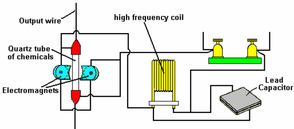
SCHEMATIC LAYOUT
