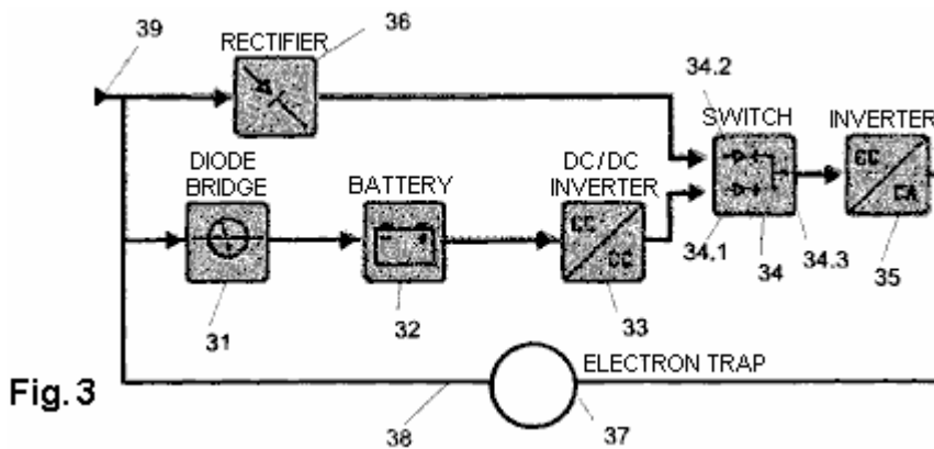
Fig.3 shows another embodiment of the self-powered system for generating electricity, comprising a device which includes the basic circuit of a typical Uninterruptible Power Supply, consisting of a battery charger (AC/DC converter) 31 connected to a drive device (inverter DC/AC) 35 and attached to them, a battery bank 32 . This basic circuit together with other devices is connected to an electron-trap 37 for collecting free electrons from surrounding space or, alternatively, an Earth-connected electron trap 37 . We have then, a bank of batteries 32 connected to the DC/DC converter 33 , which is connected to the phase transfer switch 34 / 34.1 which is connected to point 34.3 , which connects to the inverter 35 , and so, the electron-trap 37 .
