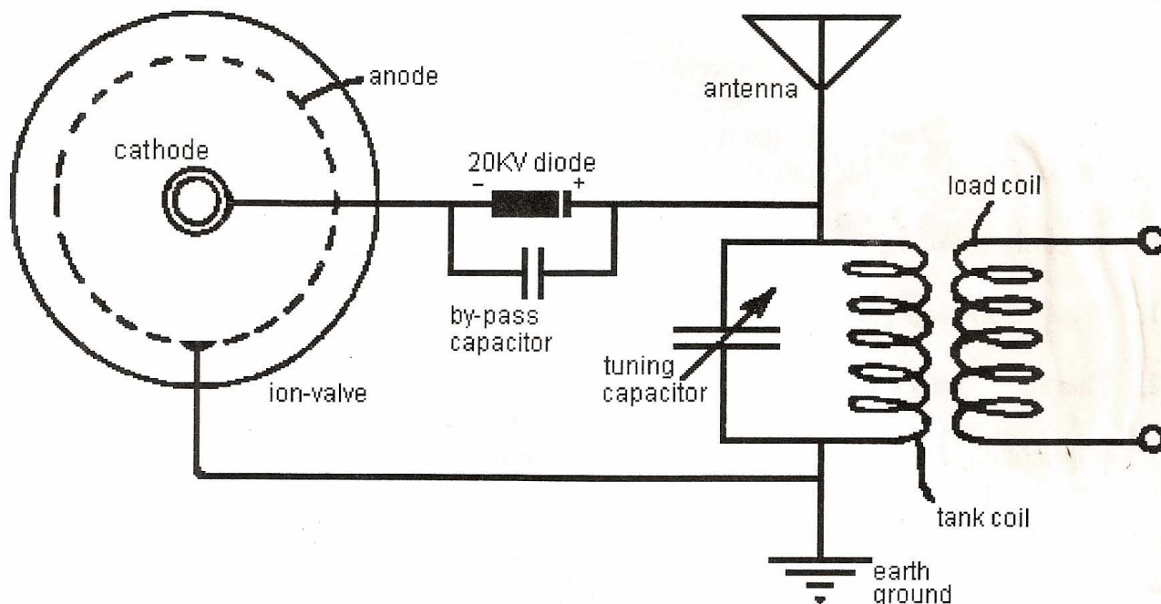
Basic Radiant Energy Receiver - Figure 3
