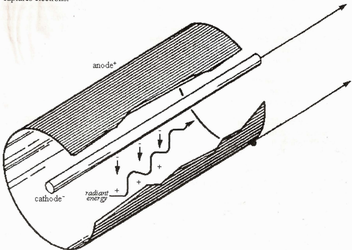
Ion Valve - Figure 4
