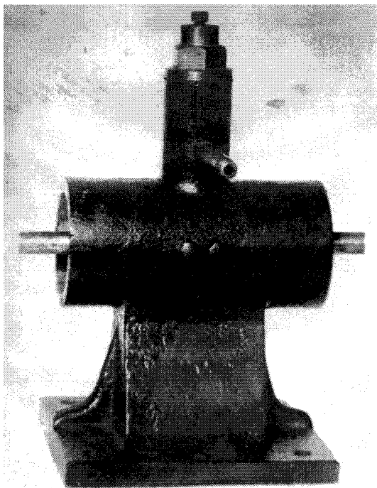
Figure 19. Simple mechanical oscillator used in first experiments.
