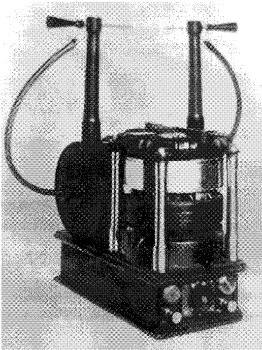
Figure 45. Hermetically enclosed mercury circuit controller with com- pact oscillatory transformer. Described in U.S. Patent No. 609,245 of August 16, 1898.
