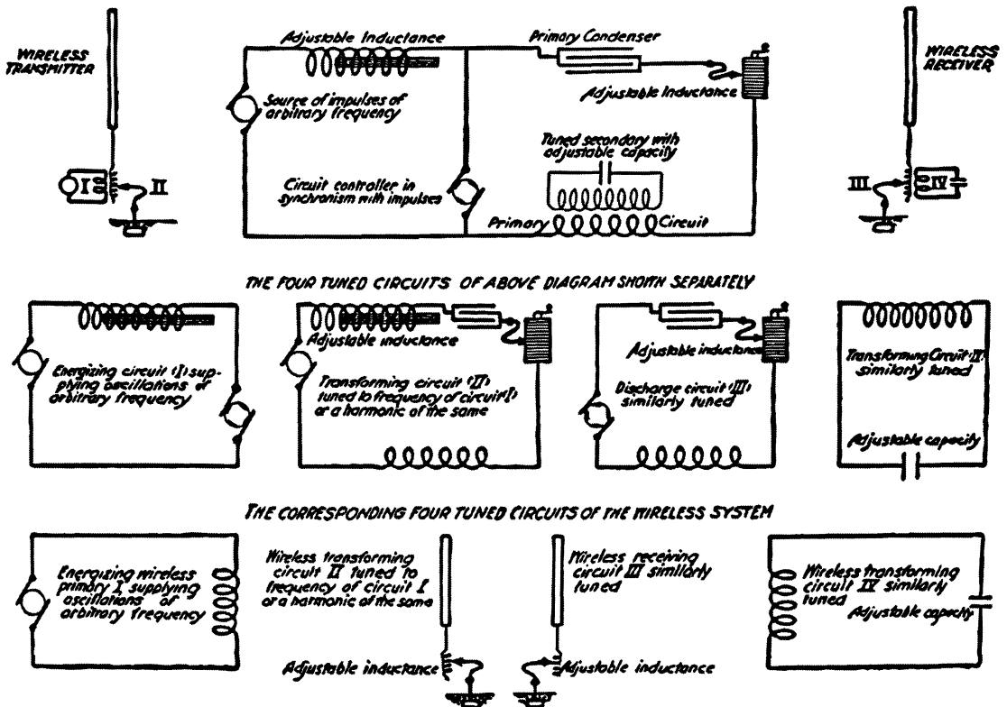
System of concatenated tuned circuits shown and described in Tesla U.S. Patent No. 568,178 of Sept. 22, 1896, and corresponding arrangements in wireless transmission
